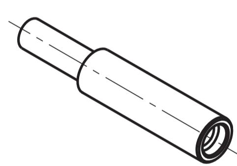
modular tie-rods L1 = 14,5 mm each place (package 100 pcs.) weight: 0,003 Kg
