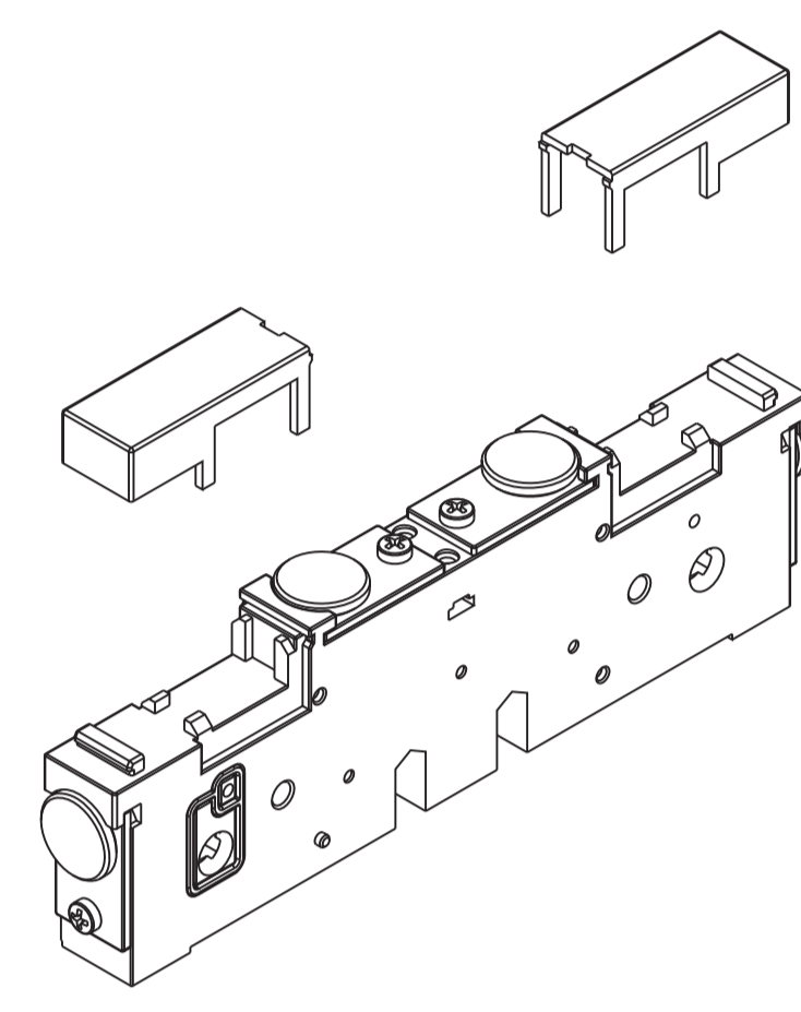
intermediate plate 14,5 mm, closed air supply and exhaust weight: 0,171 Kg
