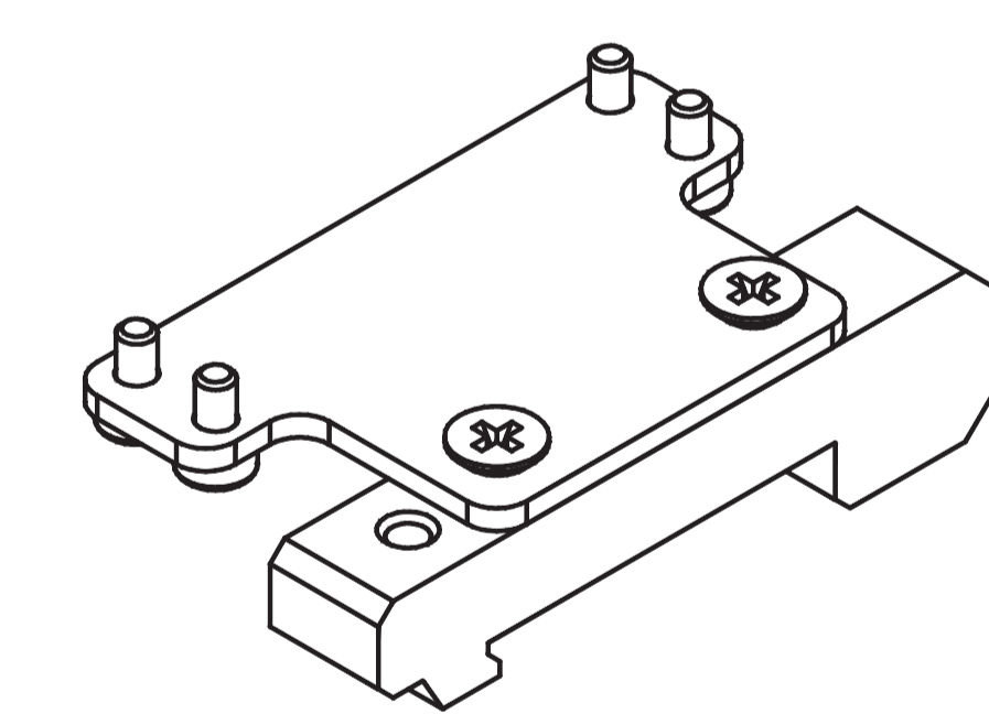
DIN rail adapter plate with screws (package 2 pcs. suitable for all models) weight: 0,066 Kg
