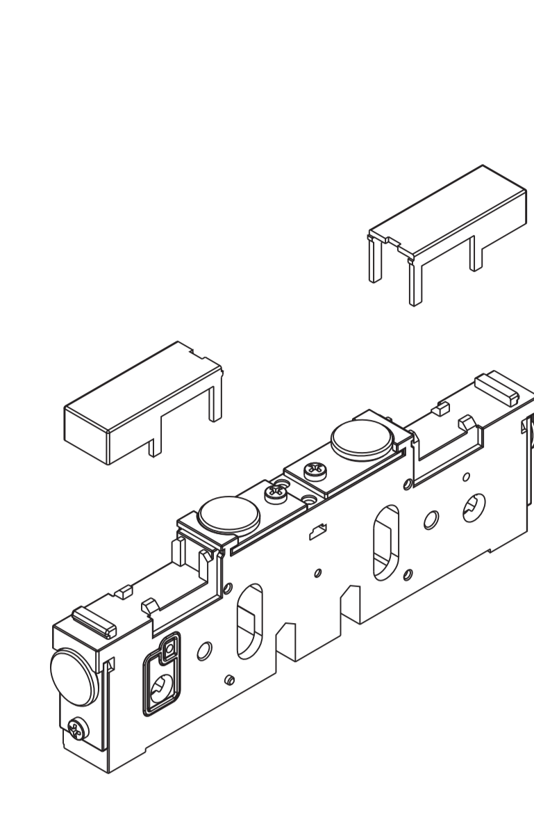
intermediate plate 14,5 mm, closed air supply, open exhausts weight: 0,167 Kg
