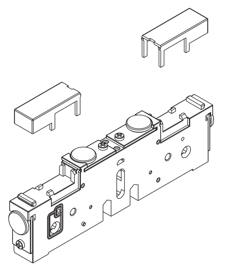
intermediate plate 14,5 mm, open air supply, closed exhausts weight: 0,170 Kg
