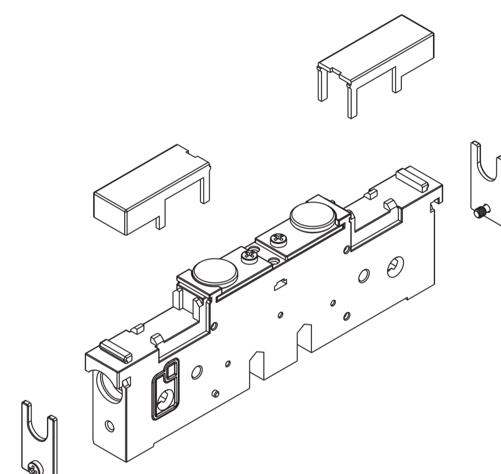
intermediate supply plate with closed exhausts and internal pilot supply weight: 0,164 Kg
