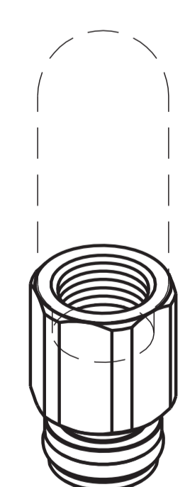
G1/8 Fitting seat reducing plug - gas thread for silencer assembly weight: 0,011 Kg
