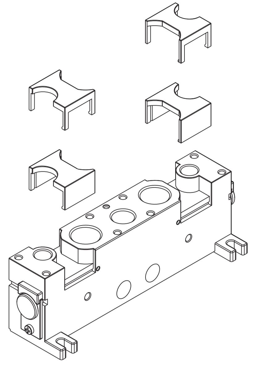
inlet plate 26 mm internal pilot supply weight: 0,295 Kg
