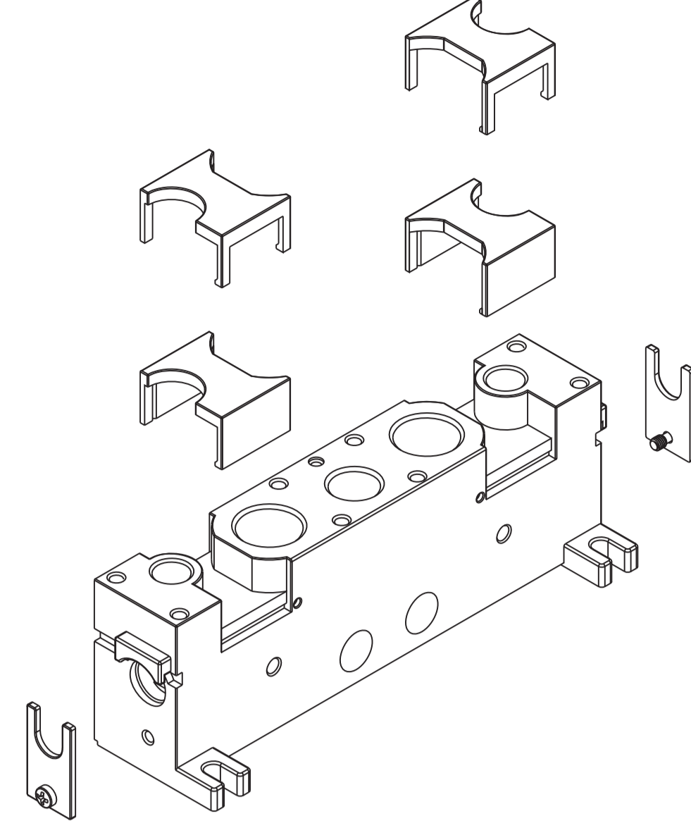
inlet plate 26 mm external pilot supply weight: 0,290 Kg
