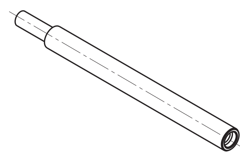
modular tie-rods L5 = 72,5 mm for 5 places (package 100 pcs.) weight: 0,015 Kg
