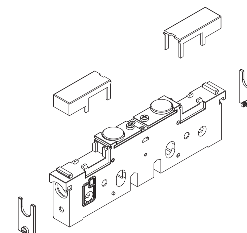
intermediate supply plate with open exhausts and internal pilot supply weight: 0,164 Kg
