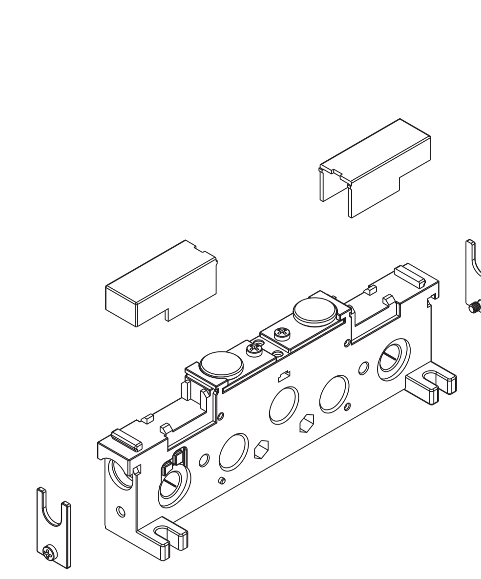
intel plate 14,5 mm external pilot supply weight: 0,162 Kg
