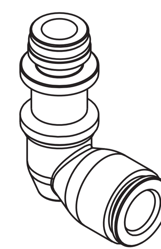
swivel low elbow fitting (package 50 pcs.) GZR-V20004 tube: 4 mm weight: 0,013 Kg GZR-V20006 tube: 6 mm weight: 0,014 Kg GZR-V20008 tube: 8 mm weight: 0,015 Kg
