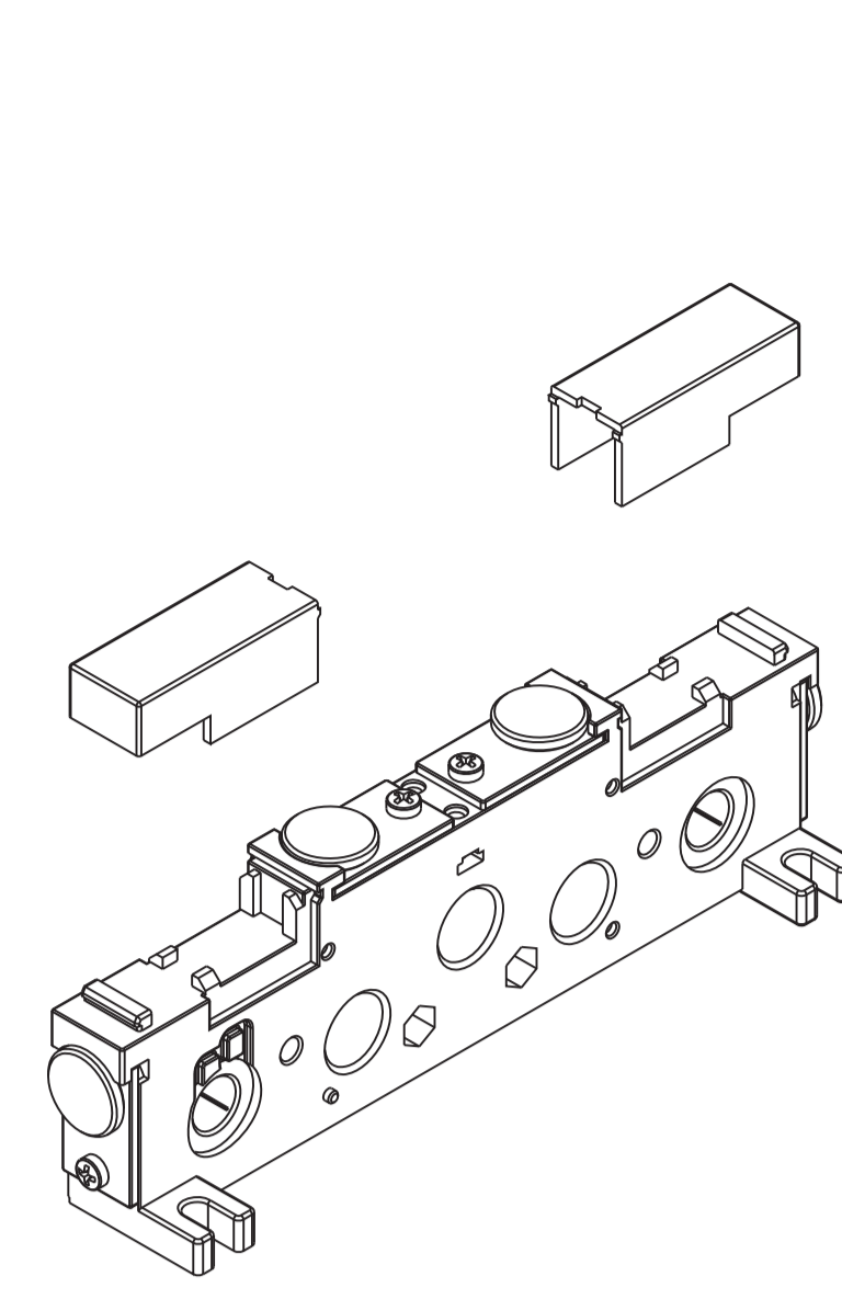
intel plate 14,5 mm internal pilot supply weight: 0,167 Kg
