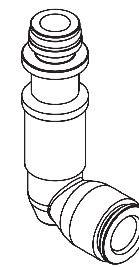
swivel high elbow fitting (package 50 pcs.) GZR-V20L004 tube: 4 mm weight: 0,017 Kg GZR-V20L006 tube: 6 mm weight: 0,021 Kg GZR-V20L008 tube: 8 mm weight: 0,027 Kg
