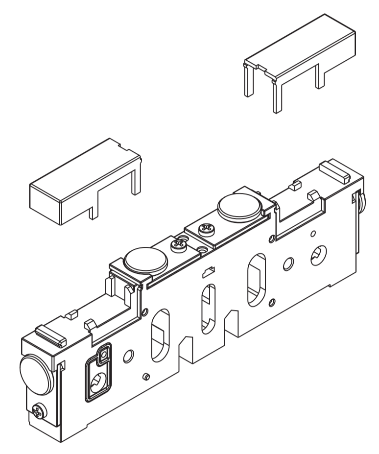
intermediate plate 14,5 mm open air supply and exhaust weight: 0,165 Kg
