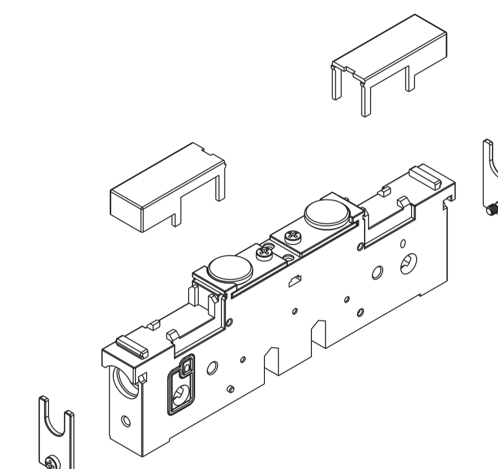
intermediate supply plate with closed exhausts and external pilot supply weight: 0,164 Kg
