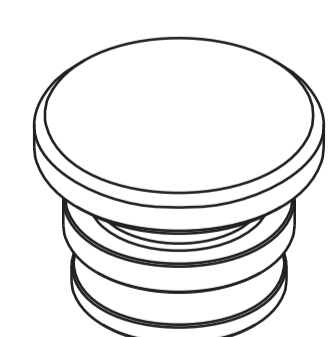
plug (package 2 pcs. suitable for all models) weight: 0,002 Kg
