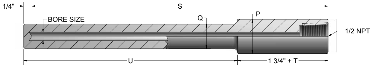
Thermowell Dimensions
