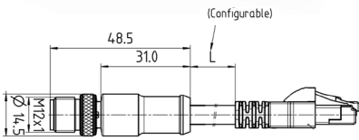
D-coded Male to RJ45 Connector
