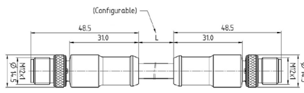
D-coded Male to Male Connector
