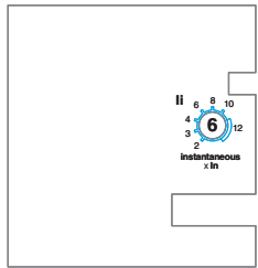
Instantaneous pickup 2~12 x I n at 800A
