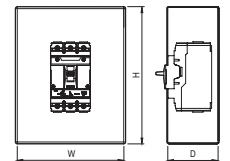
Enclosure Dimensions
