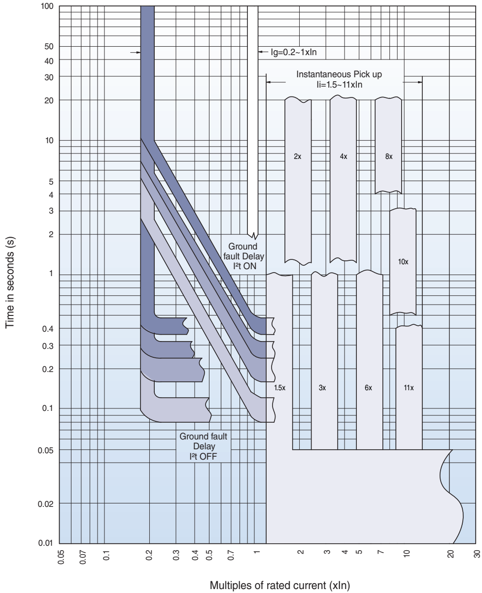
INSTANTANEOUS AND GROUND FAULT CURVE
