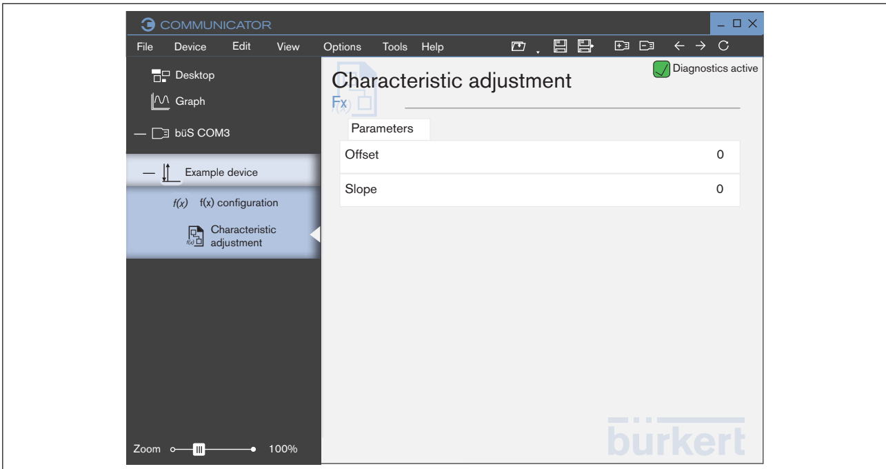
Figure 23: Adjusting parameters
