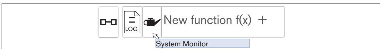
Figure 2: Tool tips
