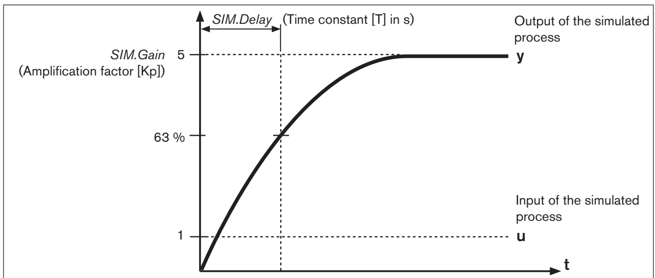
Figure 26: Example of a simulated process. Performance of the PT1 element
