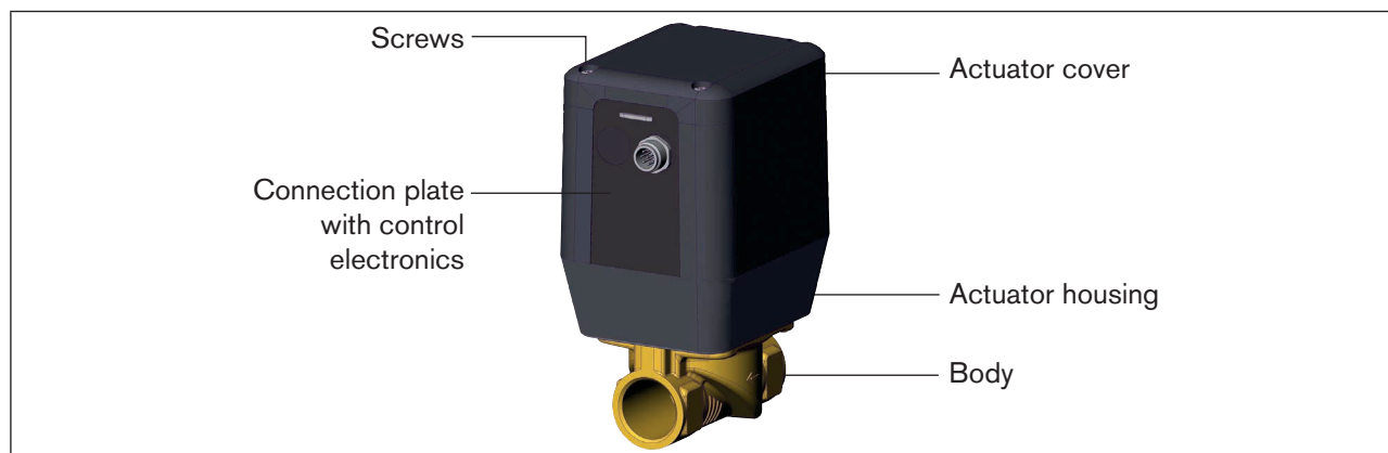
Figure 16: Opening the actuator cover, Type 3285
