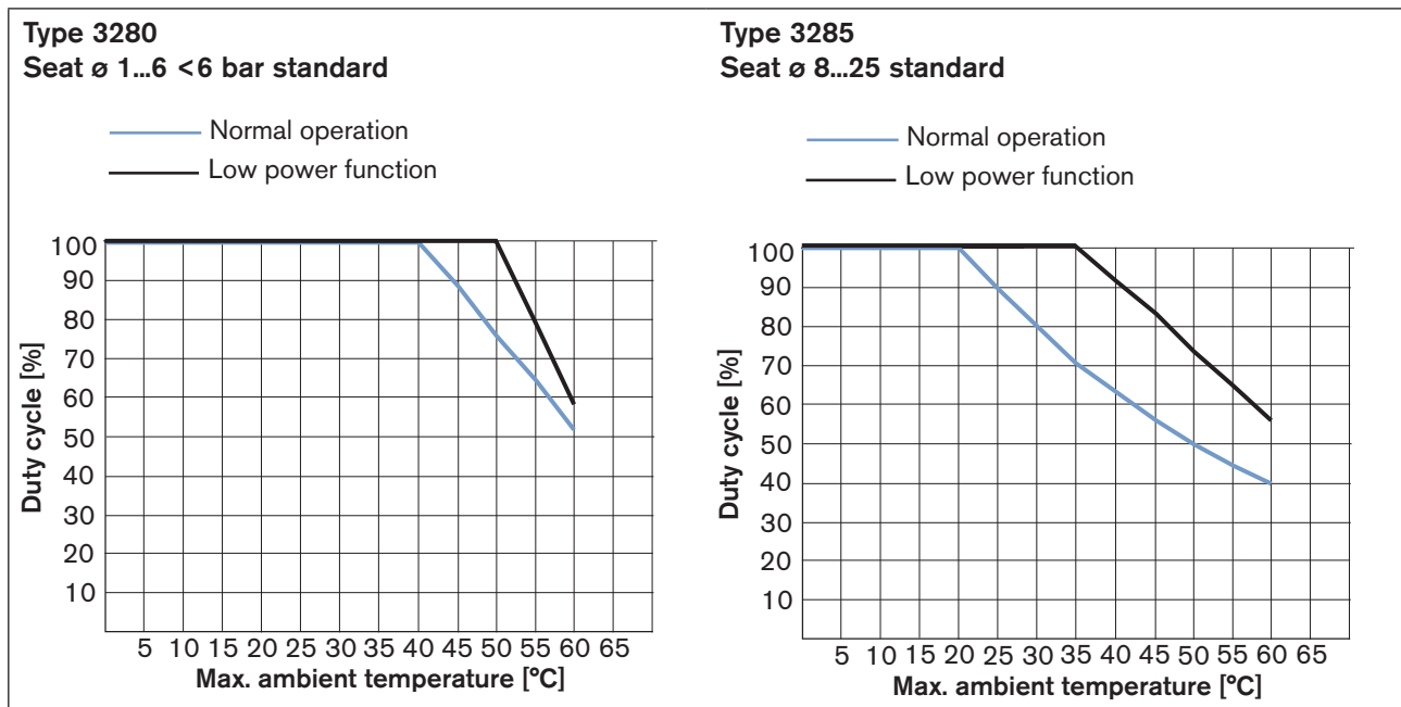
Figure 6: Derating curve for standard device
