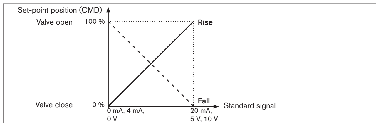
Figure 22: Graph of effective direction
