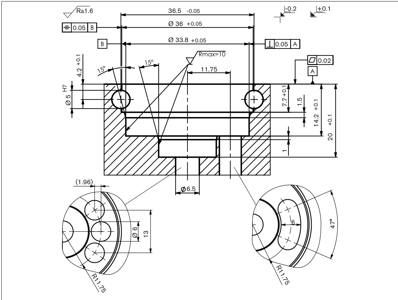
Figure 10: Installation area for cartridge body
