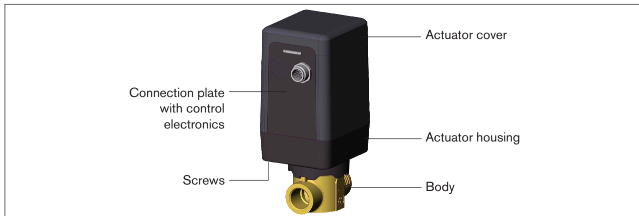
Figure 15: Opening the actuator cover, Type 3280
