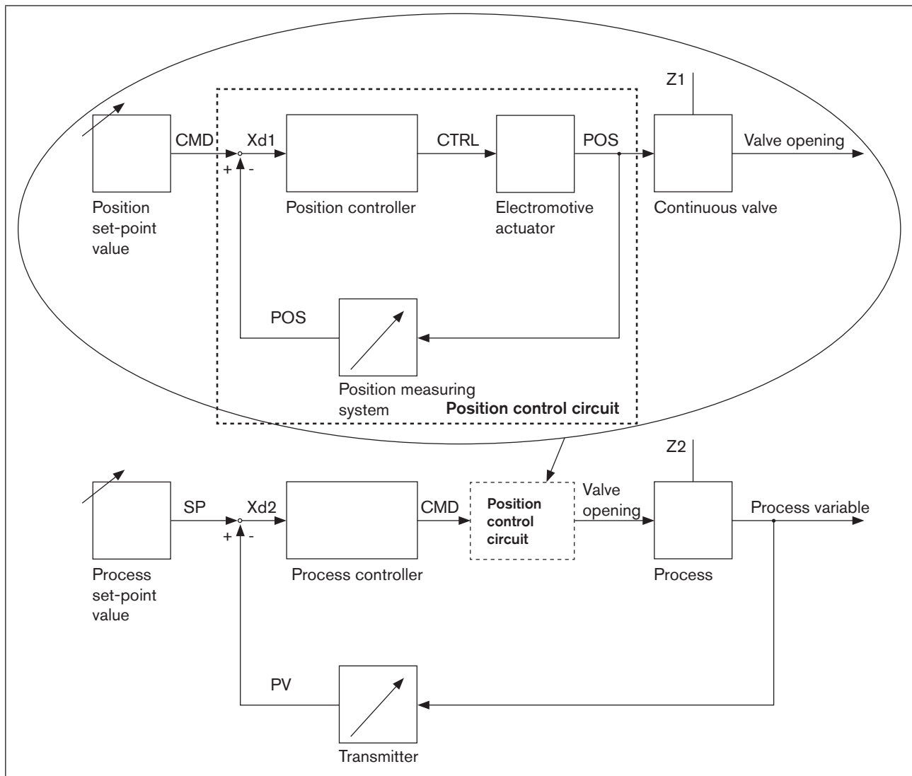
Figure 4: Signal flow diagram process controller
