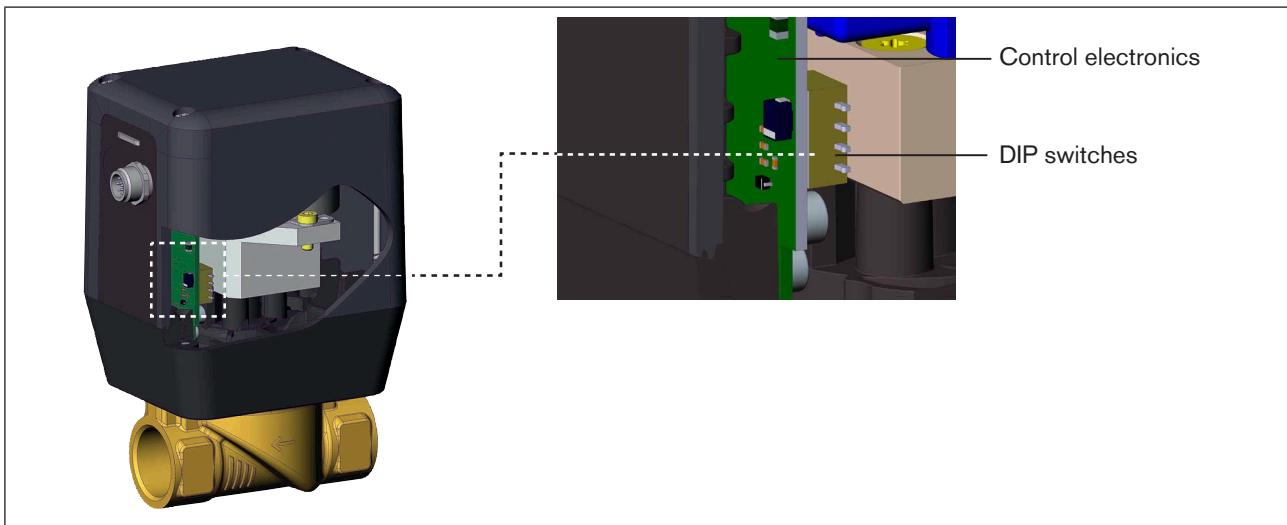
Figure 18: Location of the DIP switch for Type 3285
