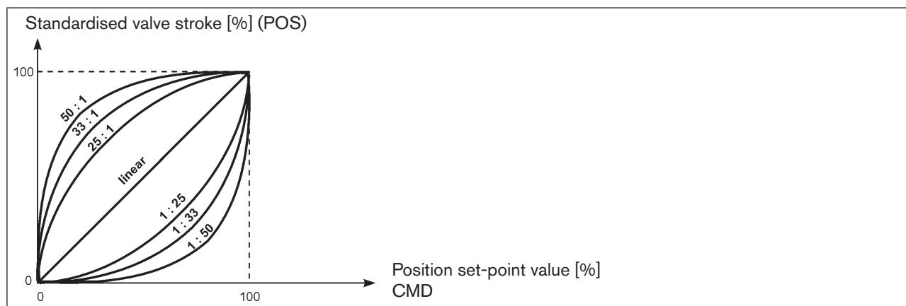
Figure 24: Characteristics
