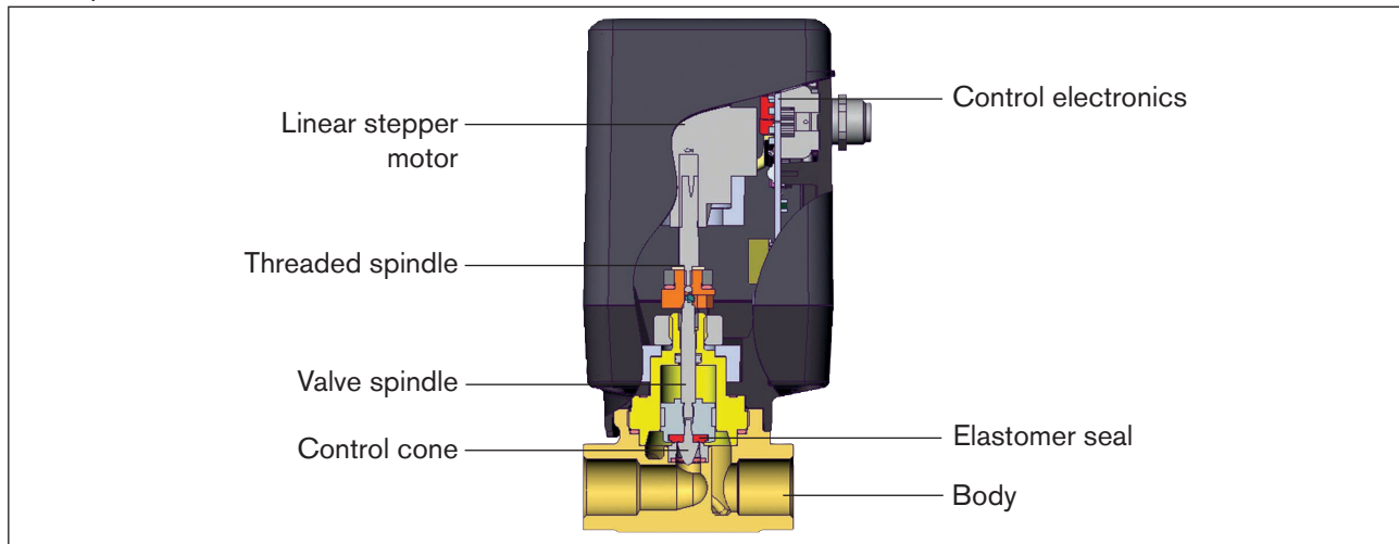
Figure 1: Electromotive seat valve Type 3280
