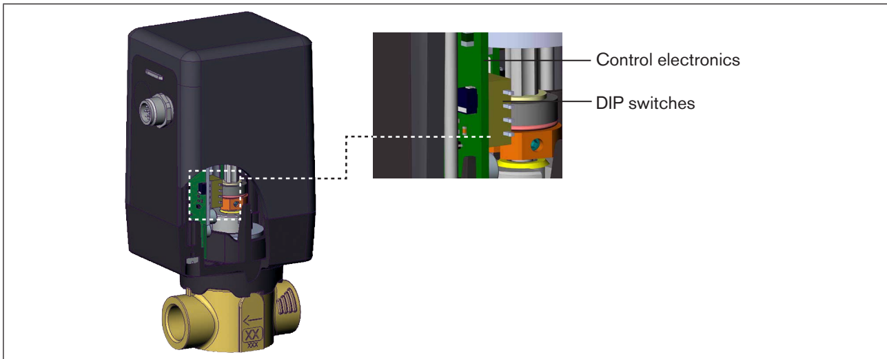
Figure 17: Location of the DIP switch, Type 3280
