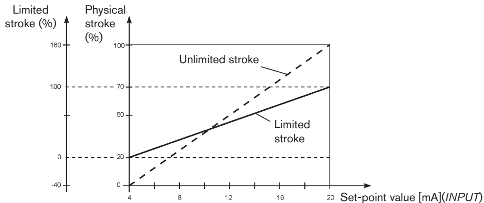
Figure 23: Diaphragm X.LIMIT
