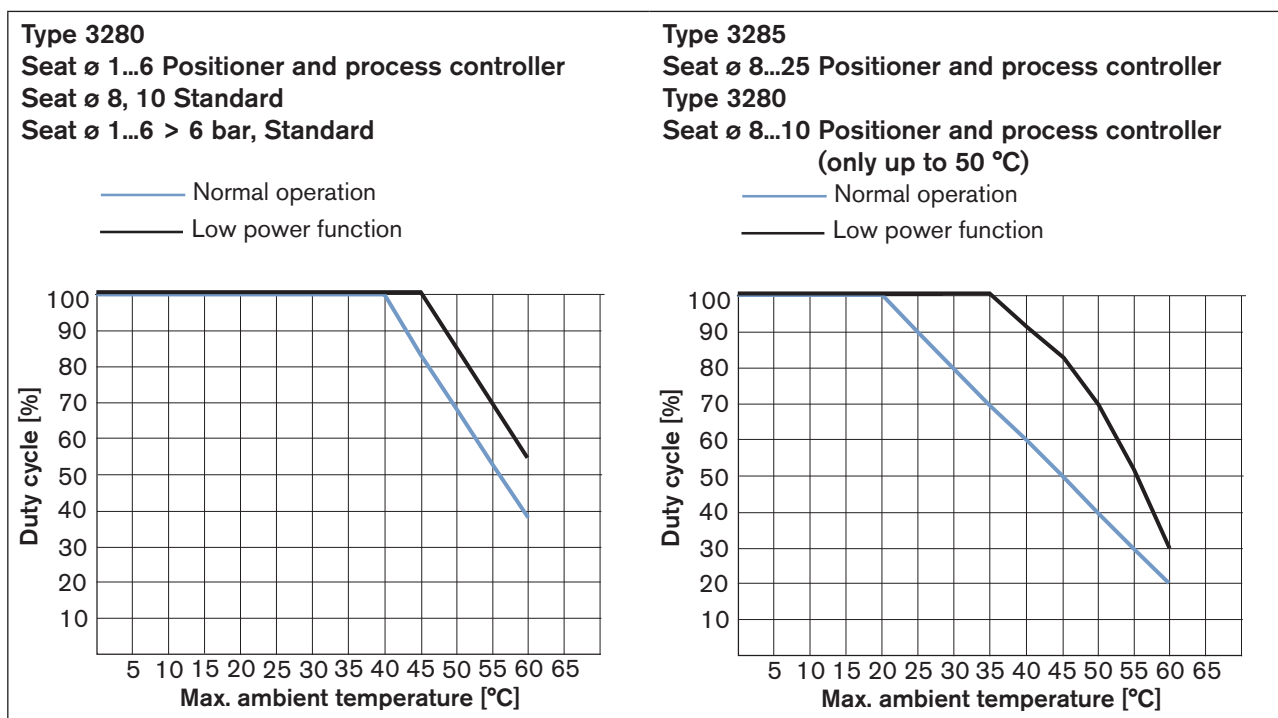
Figure 7: Derating curve for control positioner, process controller and standard version
