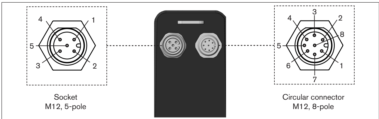
Figure 13: Designation of the circular connector, analog version
