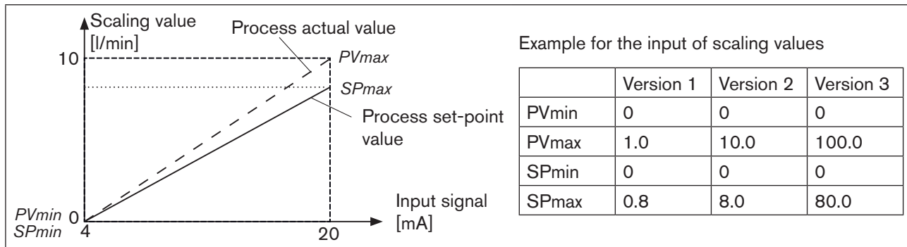
Figure 25: Example of a sensor calibration
