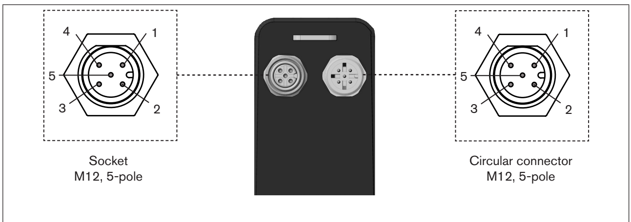
Figure 14: Designation of the circular connector, digital version
