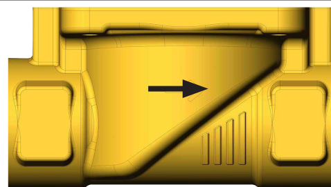
Figure 9: Direction of flow Type 3285, Flow direction above seat
