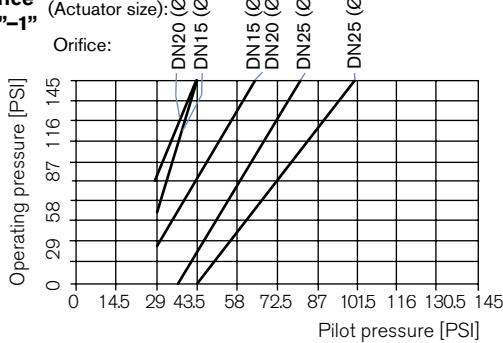
Chart 3 - orifice 1/2"-1"
