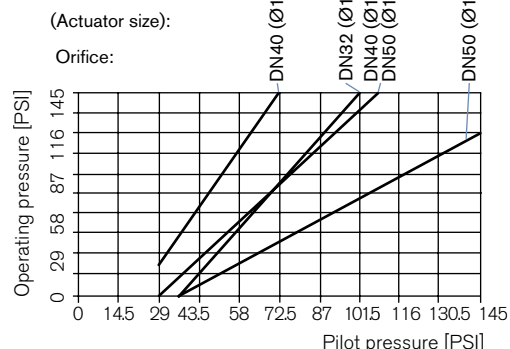
Chart 4 - orifice 1 1/4"-2"
