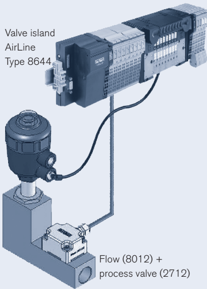
On/Off control loop
