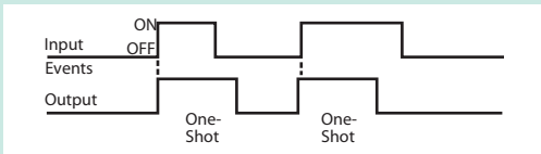
One-Shot Triggers One-Shot
