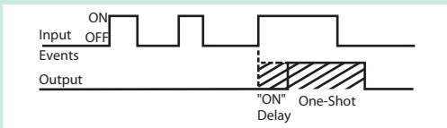
"ON" Delay, then One-Shot
