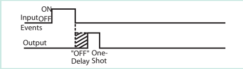
"OFF" Delay then One-Shot
