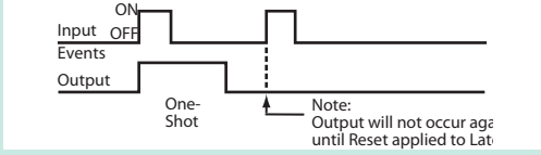
Latch, then One-Shot
