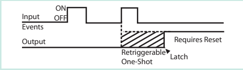
Stop Motion, then Latch
